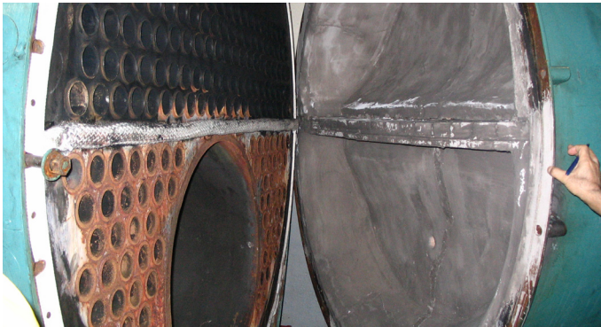
Item #1c, 1g, 2c, 2g. View showing the repaired refractory and diffuser plate inside the boiler.
